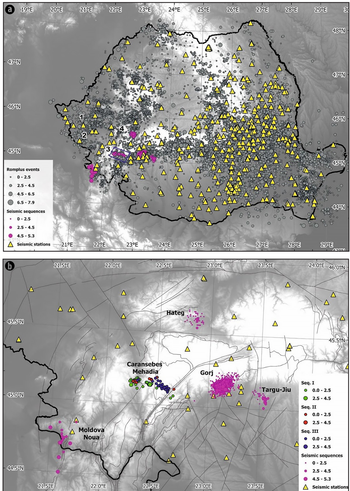
Fig. 3. (a) Seismic representation of the CMB (light blue dots inside dark blue polygon) events highlighted over the ROMPLUS events (grey dots) between 1984 and 2023 with Mw-related symbol size. The pink dots represent the seismic and swarm sequences from SWCBZ between 1889 and 2016 (Oros, 2004; Radulian et al, 2014; Placinta et al, 2016; Popa et al, 2018 and this study). Earthquake prone-clusters: (1) Sănnicoulu - Arad, (2) Timișoara and Banloc-Voiteg, (3) Oravița - Moldova-Nouă and Mehadia - Orșova, (4) Poiana Ruscă Mts - Hațeg Basin - Bistra Valley; Red polygon represents the zoom of figure 3b. (b) Sequences in the SWCBZ area: sequences 1 (green), 2 (red) and 3 (blue) in CMB and other sequences (pink). Symbol size scales with magnitude for three intervals: 0 - 2.5, 2.5 - 4.5, 4.5 - 5.5.
